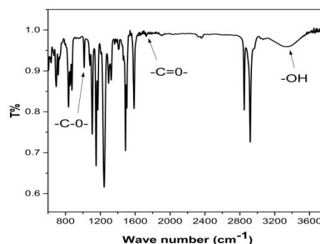
Figure 1. FTIR spectra of PVA membranes crosslinked with different malic acid content
