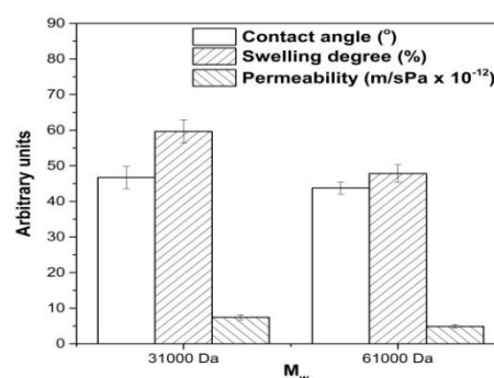
Figure 6. Contact angle, swelling degree and permeability of membranes developed by various PVA M_w
