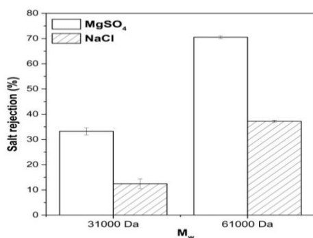
Fig 7. Effects of PVA Mw on the separation performance of prepared NF membranes
