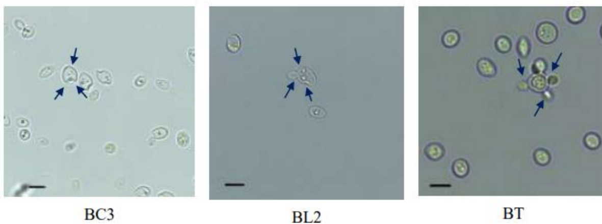
Figure 3. Location of yeast bud scars in (arrow) liquid hansen media for 20 days. Scale bar 5 µm
