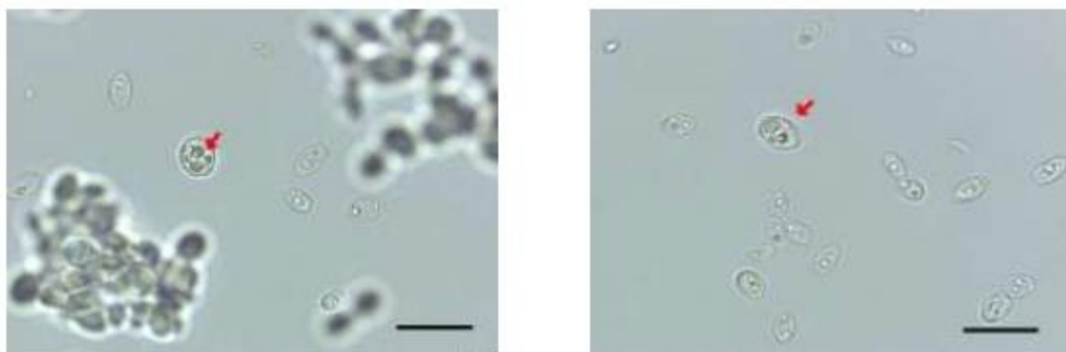
Figure 4. Morphological characteristics of asci with 4 ascospores of the yeast strain BC2.2 (arrow). Scale bar 10 \mu m
