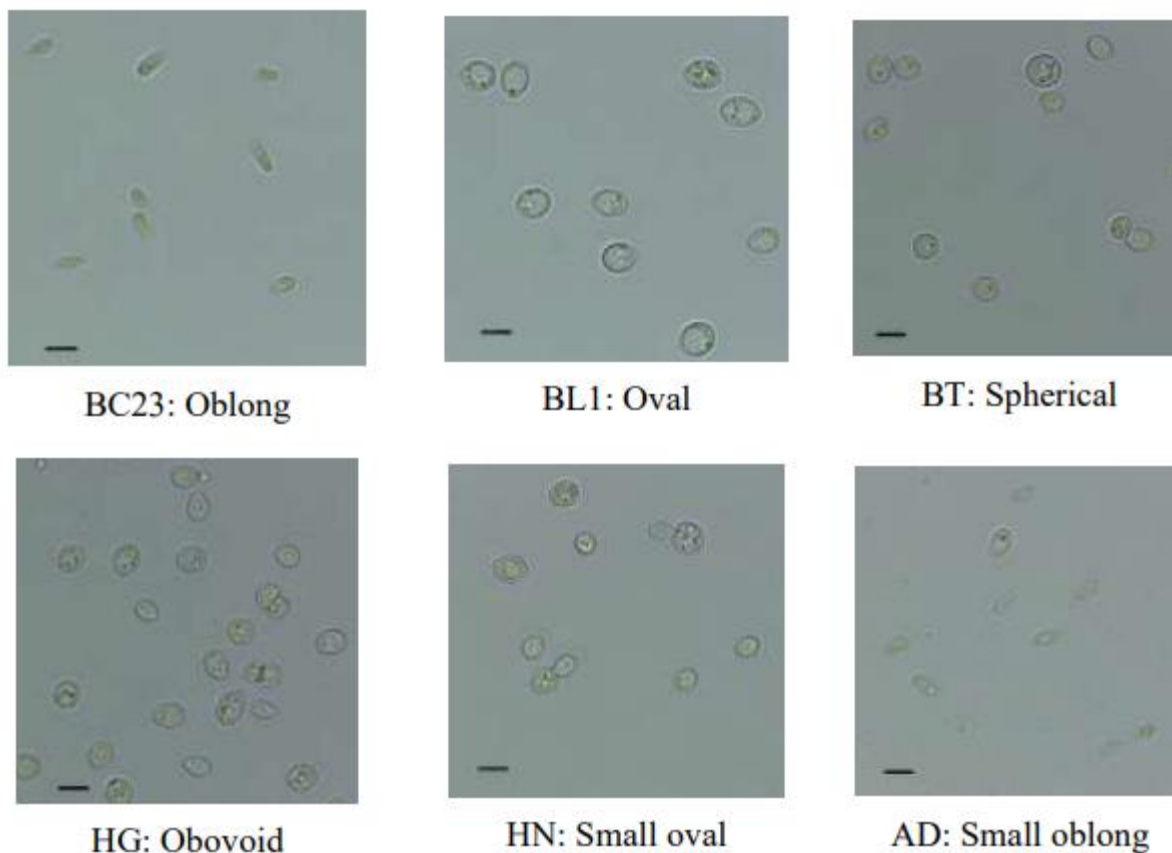
Figure 2. Types of morphological characteristics of isolated strains in liquid hansen media. Scale bar 5 µm
