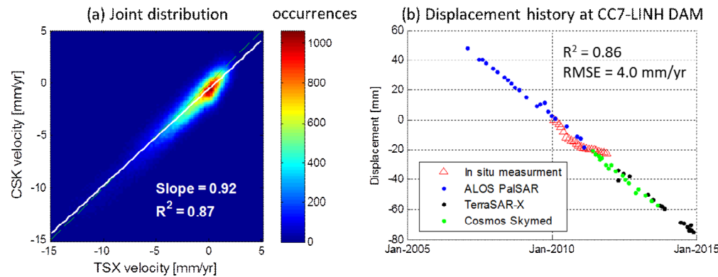
Figure 3. (a) Joint distribution between TSX velocity and CSK velocity. (b) The displacement history retrieval at CC7-Linh Dam building, where the in situ measurement is available.
