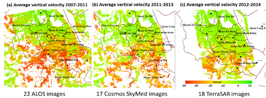
Figure 1. The average velocity trend. Positive velocities (green colors) represent movement uplift; negative velocities (red colors) represent movement subsidence.
