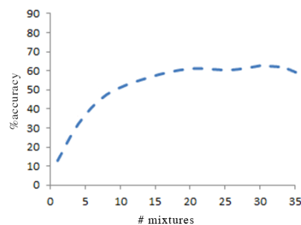
Fig. 7. Clustering performances.
