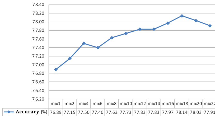
Fig. 6. Transcription performances.
