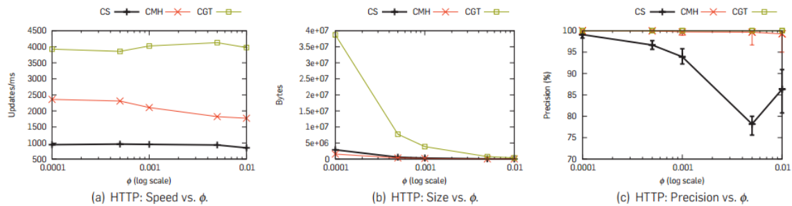
Fig. 2. Performance of sketch algorithms on real network data [24]
