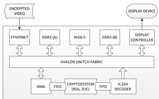
Fig. 1. The overall block diagram of the proposed embedded system
