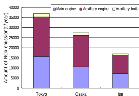
Figure 1. Amount of NOx emission in each bay
