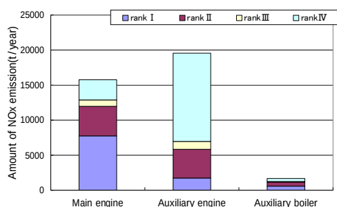
Figure 2. Amount of NO x emission of each engine category (Tokyo Bay)
