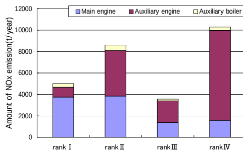
Figure 5. Amount of NO x emission of each ship size (Osaka Bay)
