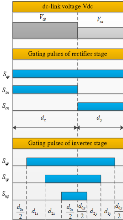
Figure 4. Transistors' gating pulses when the input current and output voltage reference vectors are assumed to be both lying within sector 1.
