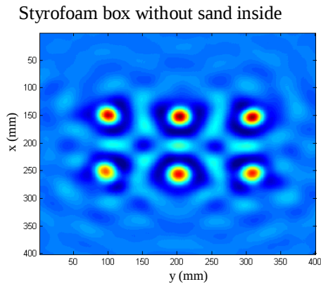
Figure 23. Applying HS algorithm for the case six metal sticks in styrofoam box without sand inside
