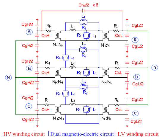
Figure 2. Lumped circuit of a Yy6 transformer
