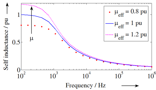
Figure 6. Influence of \mu_{eff} on a calculated normalized inductance ( \rho_{eff} unchanged)
