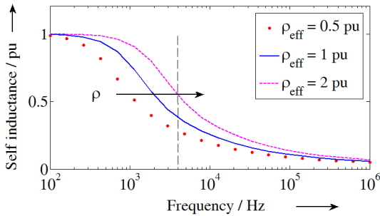
Figure 7. Influence of \rho_{eff} on a calculated normalized inductance ( \mu_{eff} unchanged)
