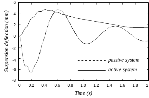
Fig. 8. Suspension deflection with step disturbance
