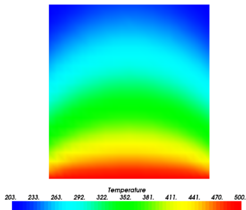
Figure 14. The temperature distribution in the square plate with 961 DOFs base on FEM and 49 DOFs base on cubic IGA
