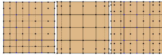
Figure 9. Quadratic, cubic and quartic mesh
