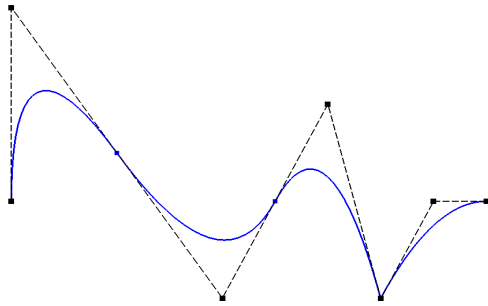
Figure 7. B-spline, piecewise quadratic curve in \square . Basis function and knot vector as in Figure 1. Control point locations are denoted by \blacksquare , and the knots, which define a mesh by partitioning the curve into elements, are denoted by \bullet .
