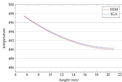
Figure 27. The temperature distribution in the fin
