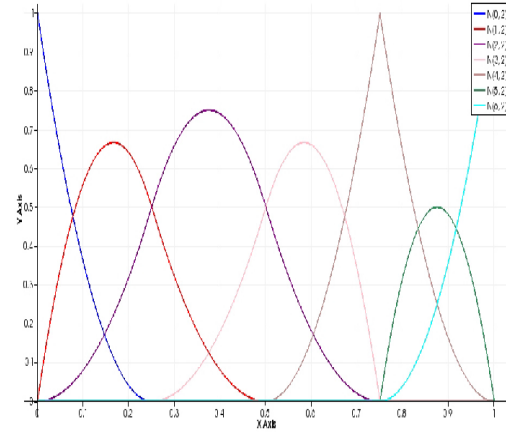
Figure 6. Quadratic basis functions for the open knot vector \Xi = \{0, 0, 0, 0.25, 0.5, 0.75, 1, 1, 1\}
