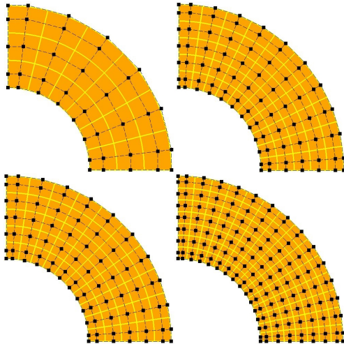
Figure 19. The refined mesh with 3 \times 6 , 5 \times 10 , 7 \times 14 and 10 \times 20
