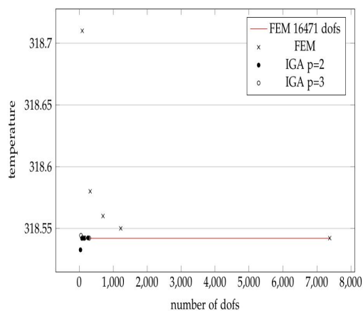
Figure 20. The convergency of temperature of point at the end of line r0, located at r = 0.15 (m) and \alpha = 90^\circ .
