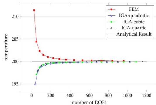
Figure 10. The comparisons of convergence of the temperature at the center of square plate
