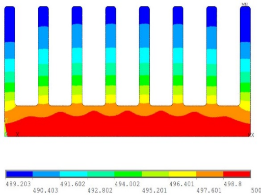
Figure 26. The temperature distribution of finite element method with about 57000 degrees of freedom
