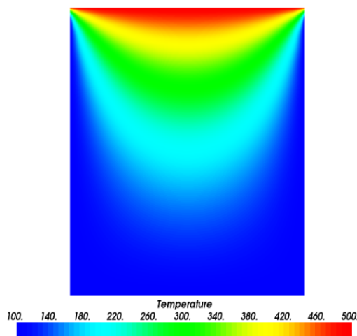
Figure 12. The temperature distribution with 961 DOFs in FEM and 361 DOFs in IGA
