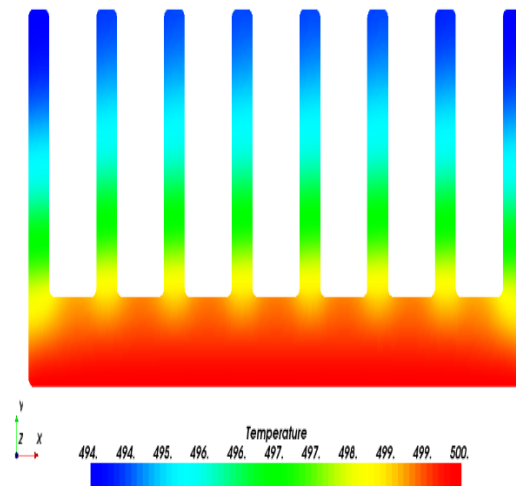
Figure 25. The temperature distribution of isogeometric analysis with about 1327 degrees of freedom
