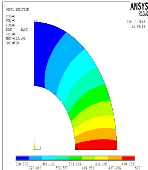
Figure 22. The contour of temperatures using FEM with 16471 dofs
