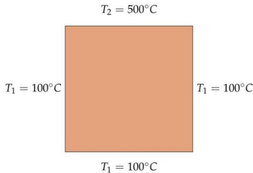
Figure 8. Square plate with boundary conditions
