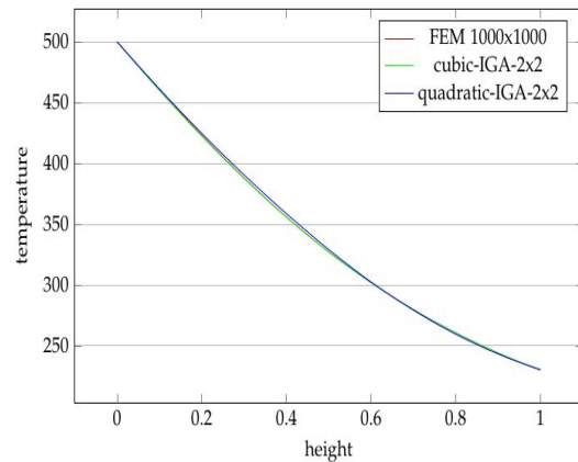
Figure 16. The temperature distribution on y direction
