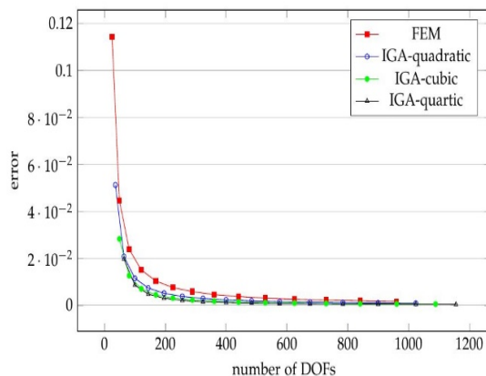
Figure 11. The error value to the analytical solution of each case
