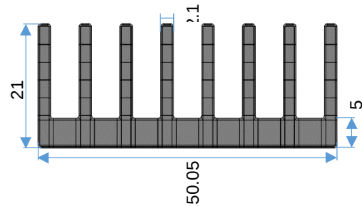
Figure 24. The heat sink model presented by NURBS surfaces
