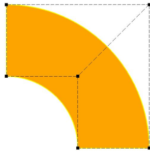
Figure 18. The coarse mesh of annular with only one element.
