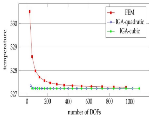
Figure 15. The comparisons of convergence of the temperature at the center of square plate with component of Neumann and Dirichlet Conditions
