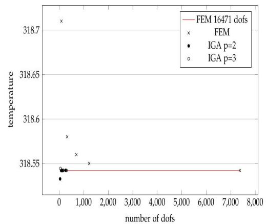
Figure 20, the convergence of IGA ( p=2 ) is better than FEM clearly. The result of FEM really accurate when number of DOFs have increased more than 1000 DOFs, while IGA just need more than 100 DOFs.
