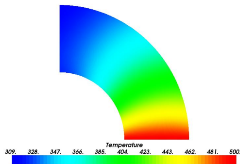
Figure 23. The contour of temperature using IGA with 231 dofs
