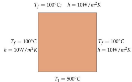
Figure 13. Square plate with both Dirichlet and Neumann boundary conditions
