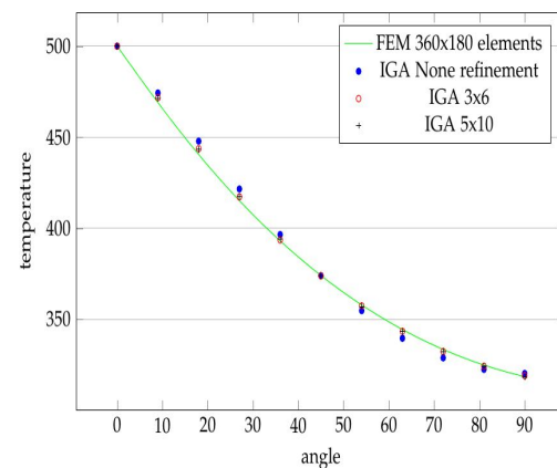
Figure 21. The convergency of temperature in line r0 for comparison of FEM with 360 \times 180 elements.
