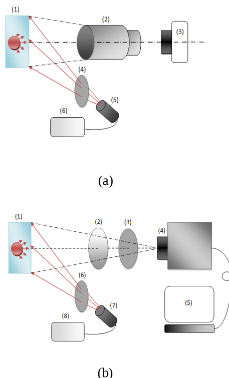
Figure 1. Schematic diagrams of the experimental setup used for fluorescence photography (a) and fluorescence spectroscopy (b).
