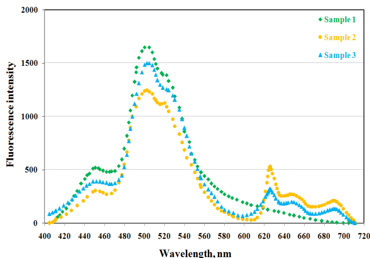
Figure 7. Fluorescence spectra of samples.
