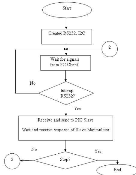
Fig 7. The flowchart on the circuit PICMaster 18F4450
