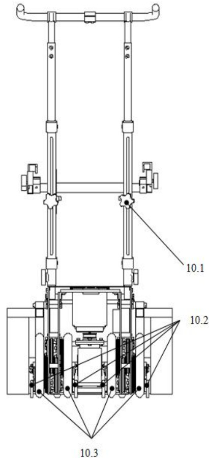
Figure 10. Machine shape from rear view
