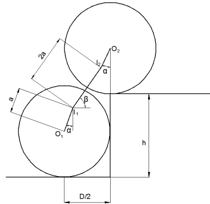
Figure 13. Dimensions of big wheels unit
