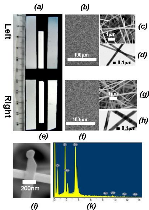
Figure 10. Optical microscopes image of SnO 2 NWs on the Si and Al 2 O 3 substrates (a, e), FE-SEM and TEM images of SnO 2 NWs (b, c, d, g, h, f) obtained on the left and right of source, (i) SnO 2 nanowires with Au catalyst cap, and (k) EDX spectrum measured at the catalyst cap [27].
