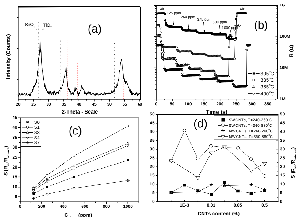
Figure 3. X-ray diffraction pattern of SnO 2 -TiO 2 shows the peaks of solid solution (a); sensor response to a serial of ethanol concentration at different temperatures (b); response versus on ethanol concentration characteristics in the range from 125 to 1000ppm at operating temperatures of 240°C; sensor response versus MWCNTs and SWCNTs inclusion content [18].
