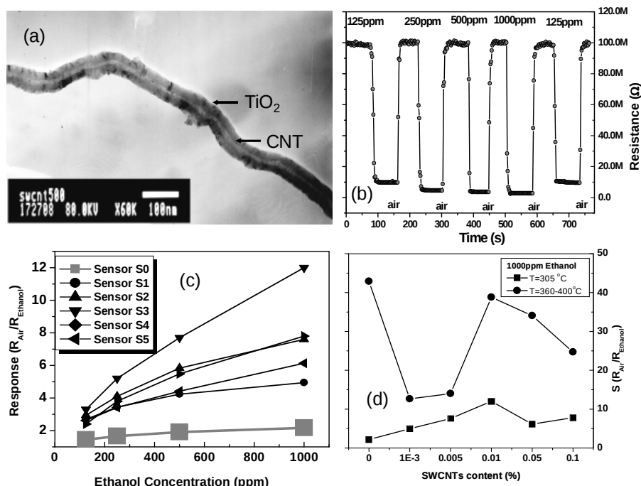
Figure 1. TEM image of morphology of CNTs-doped TiO 2 (a), Transient response of CNTs-doped TiO 2 sensor to a serial ethanol concentrations (b), sensor response versus ethanol concentration (c), sensor response versus SWCNTs-doped TiO 2 (d) [16].
