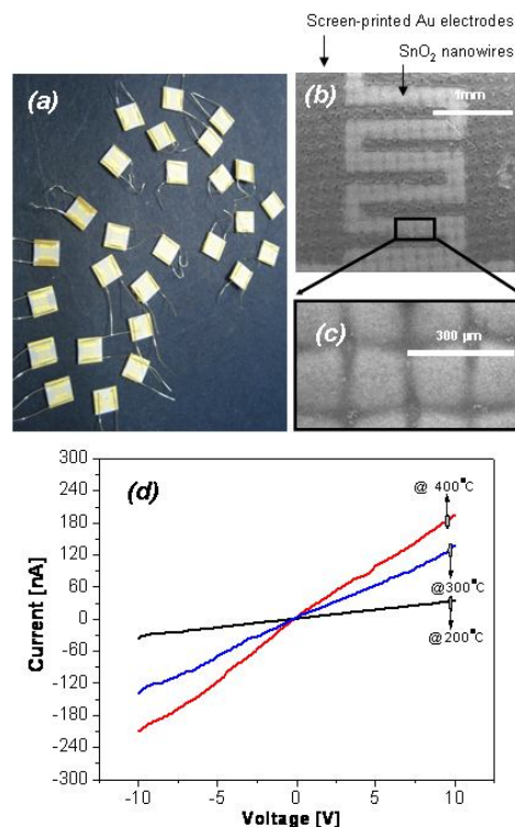
Figure 11. As-fabricated gas sensors (a,b,c) and I-V characteristic of the sensors at different temperatures (d) [27].
