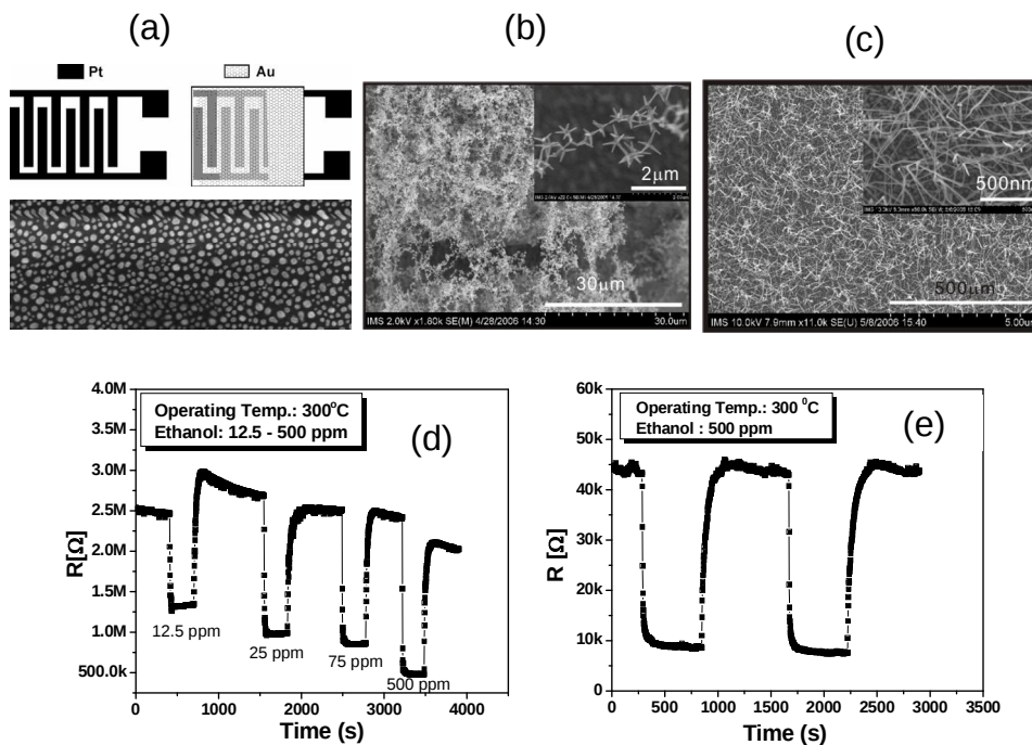
Figure 8. Interdigitated electrode with Au catalysis layer on the top (a); The ZnO nanotetrapods (b) and nanowires grown on the electrode; ethanol response of ZnO nanotetrapods- and nanowires -based sensors (d, e)[24].
