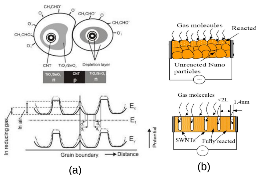
Figure 7. Schematic of potential barriers to electronic conduction at grain boundaries and at p–n heterojunctions for CNTs/SMO; d_1 and d_3 are depletion layer widths when exposed to ethanol; d_2 and d_4 are depletion layer widths in air (b); nanochannel forming the SMO materials (b) [18].
