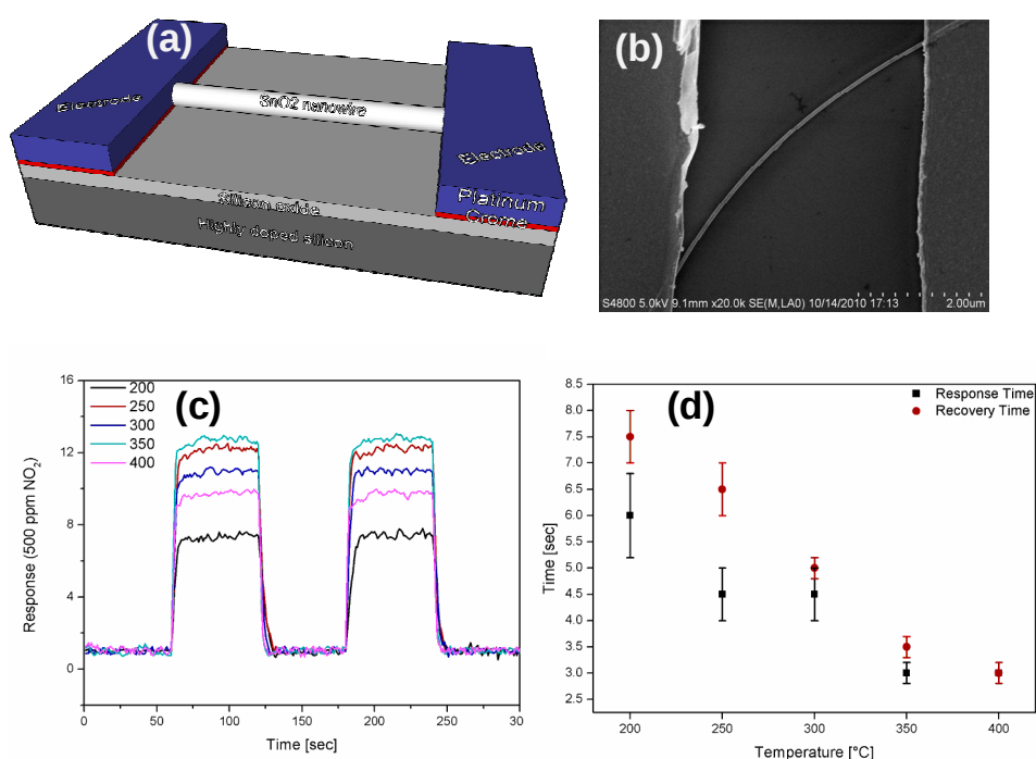
Figure 14. The configuration of single NWs gas sensor (a); As-fabricated \text{SnO}_2 NWs devices (b); the response to \text{NO}_2 at different temperatures (c); and the estimation of response-recovery time [32].
