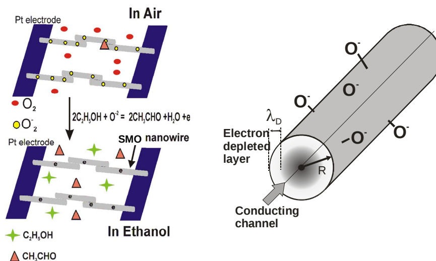
Figure 16. Summaries of gas sensing mechanism of SMO nanowires.
