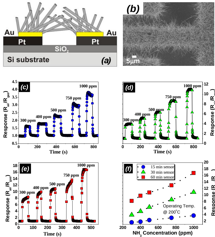
Figure 13. Schematic diagram of on-chip fabrication \text{SnO}_2 NWs sensors (a) typical SEM images of on-chip fabrication \text{SnO}_2 NWs grown for 15min (b); the change in response ( R_{\text{air}}/R_{\text{gas}} ) upon exposure to different concentration of \text{NH}_3 measured at 200^\circ\text{C} for nanowires grown at (a) 15min, (b) 30min, (c) 60min, a their response as a function of \text{NH}_3 concentration (d) [26].
