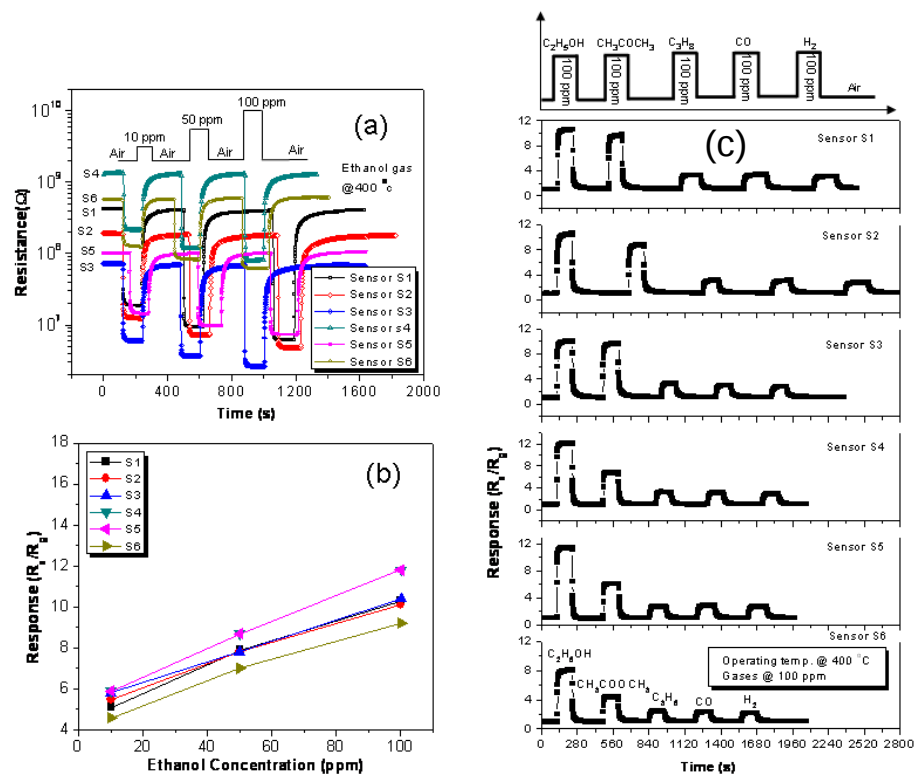
Figure 12. Response characteristic of randomly tested sensors to various ethanol concentrations at temperature of 400°C(a); response as a function of ethanol concentration (b); Transient response of randomly selected sensors to 100 ppm various gases ( C_2H_5OH , CH_3COOCH_3 , C_3H_8 , CO , H_2 ) (c) [27].
