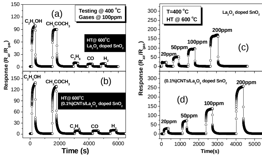
Figure 6. Sensor response of SnO 2 doped with La 2 O 3 and co-doped with CNTs to different gases (a, b) and to various ethanol concentration gas (c,d) [21].
