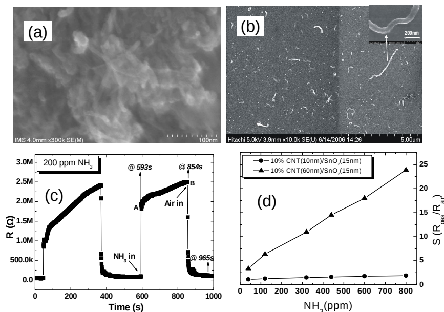
Figure 4. SEM images of SnO 2 -(10%wt)MWCNTs powder (a) and thin film (b) nanocomposites annealed at 550°C in the vacuum at 10 -2 torr; a dynamic response of the composite sensor to NH 3 gas at room temperature (c); the sensor response versus NH 3 concentration for the composite using CNTs with diameter (d) [19].
