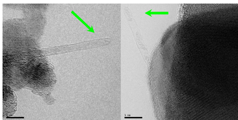
Figure 8. TEM images of SWNTs without catalytic particles at the SWNTs' top
