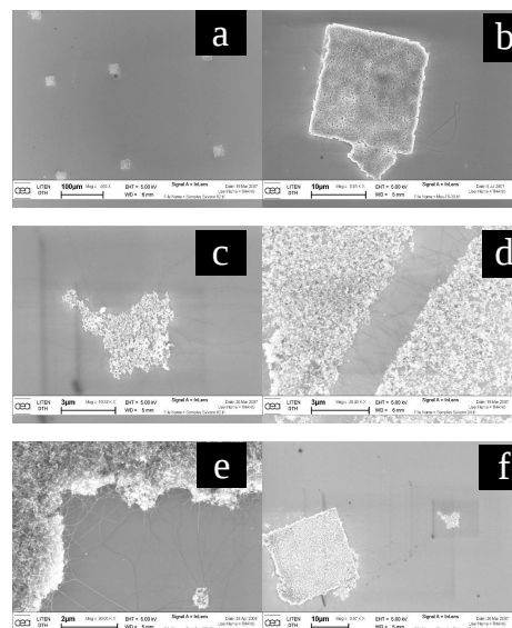
Figure 3. Scanning electron microscopy images of as-grown CNTs on/near catalyst islands
