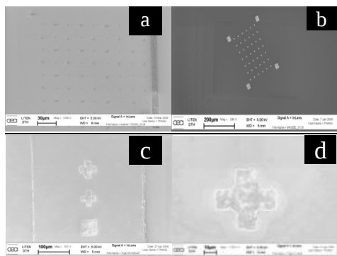
Figure 2. SEM images of markers (a) and patterned catalyst (b, c, d).
