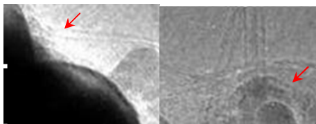
Figure 7. A typical HRTEM images of the SWNTs' bottoms
