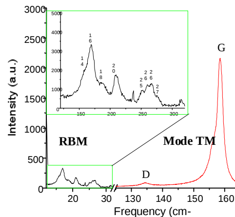
Figure 5. Raman spectroscopy of CNTs products
