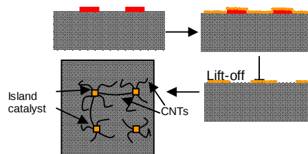
Figure 1. Patterned growth of CNTs
