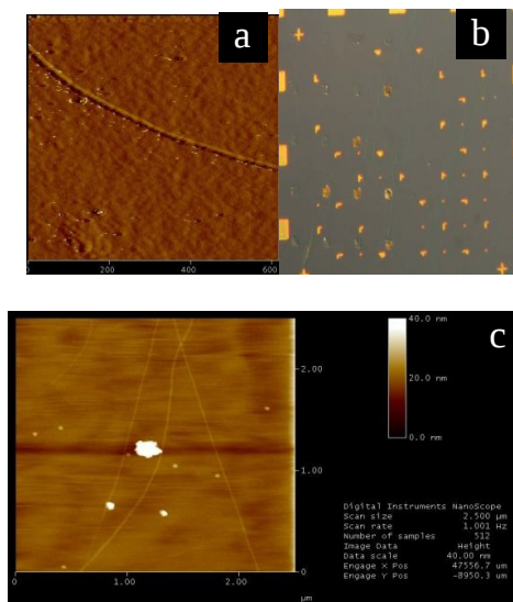
Figure 4. AFM images of as-grown CNTs from a patterned catalyst (with AFM markers)
