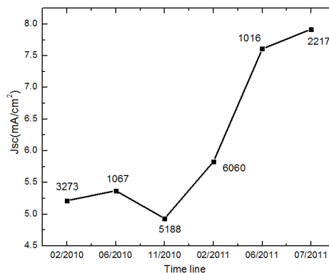
Figure 10. Short circuit current improvement; 2217 sample with ITO coating has the best J SC
