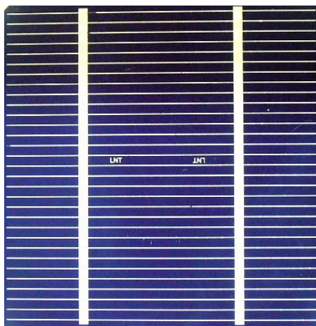
Figure 9. 2217 Solar cell, with front contact optimization, texturization and ITO antireflection coating ; \eta = 12.81\%
