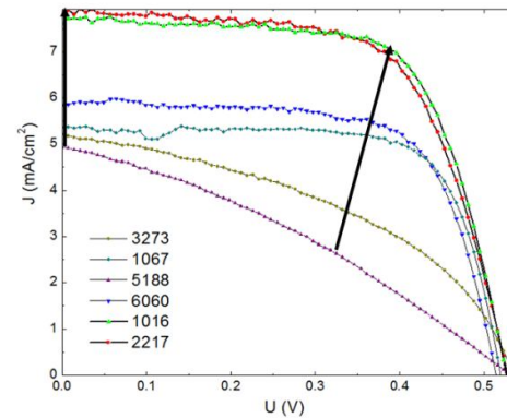
Figure 8. The short circuit improvement; 1016 ( \text{SiN}_x ) and 2217(ITO) are the best cells due to their best short circuit currents. All measures were under 21 \text{ mW/cm}^2 of irradiation.
