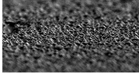
Figure 7. SEM image of random pyramids structure after the TMAH surface treatment
