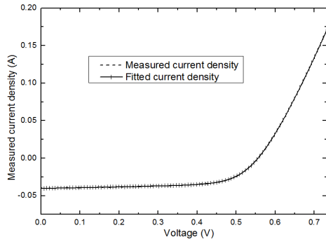
Figure 5. JV curves of the cell ID 2217 (the fitting curve with symbols using orthogonal distance regression method). The small deviation between fitted and measured curve proves the reliability of extracted parameters.
