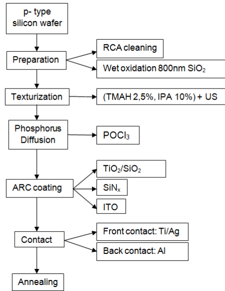
Figure 3. The solar cell fabrication process at LNT
