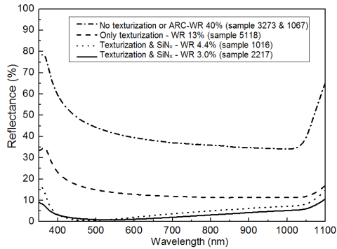
Figure 6. Influence of texturization and ARC on the reflectance spectra
