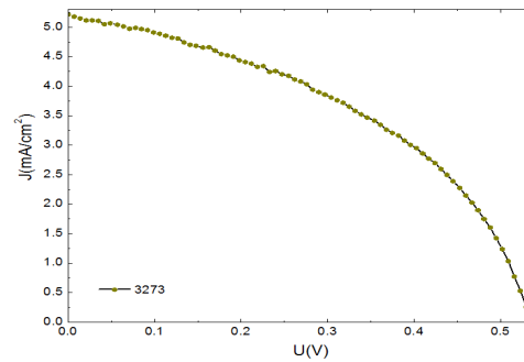
Figure 4. JV curves of cell ID 3273, the simplest cell with bad cell resistances and the high front surface reflectance and front surface recombination
